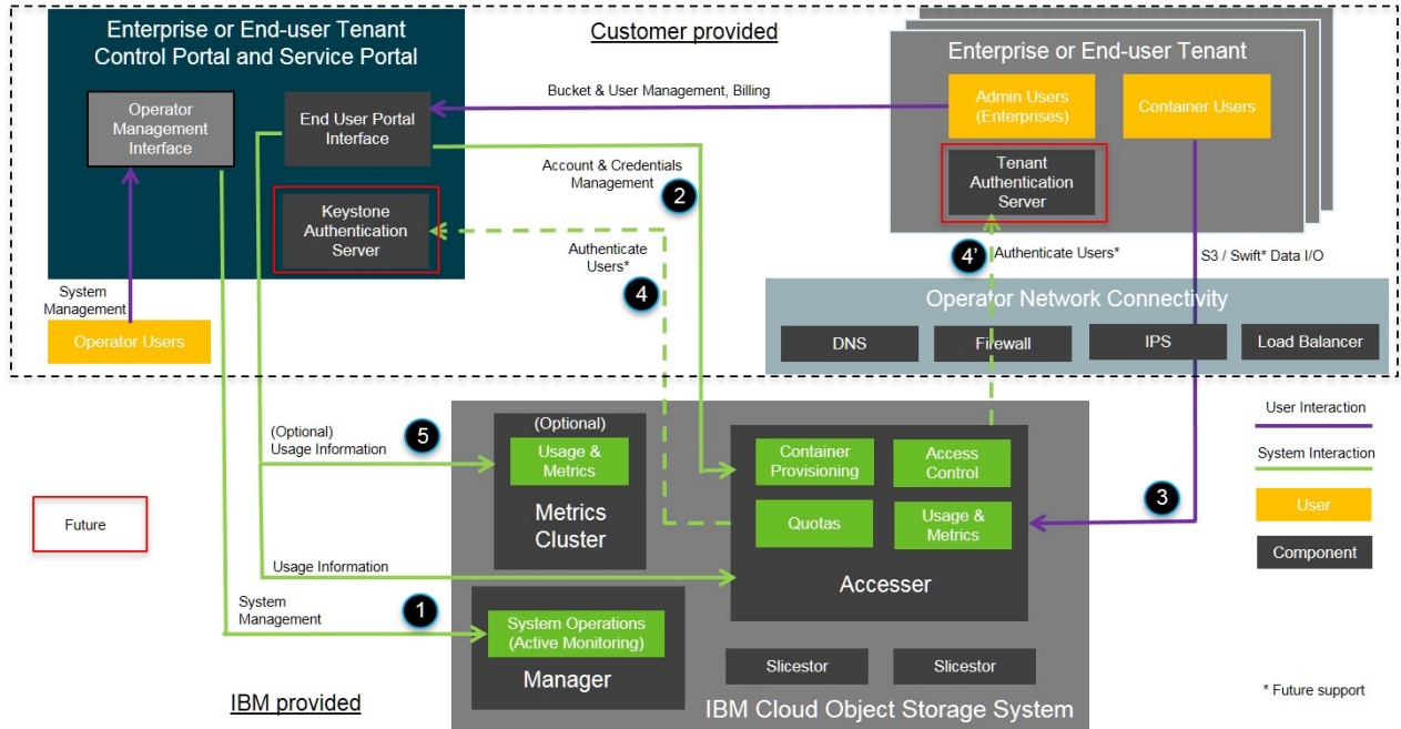
Figure 1. End-to-end STaaS system architecture
